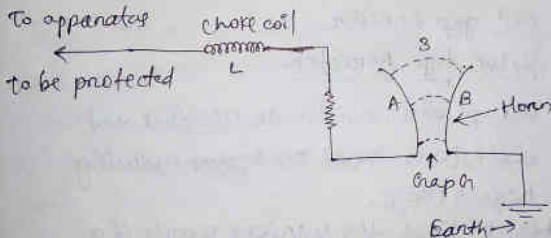
[Fig. ① Horn-gap Arrester]
